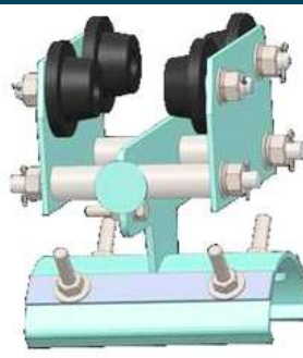
CABLE TROLLEY S Loading Capacity 60 KG Max
